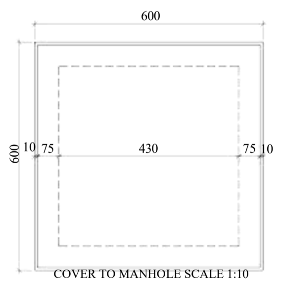
COVER TO MANHOLE SCALE 1:10
