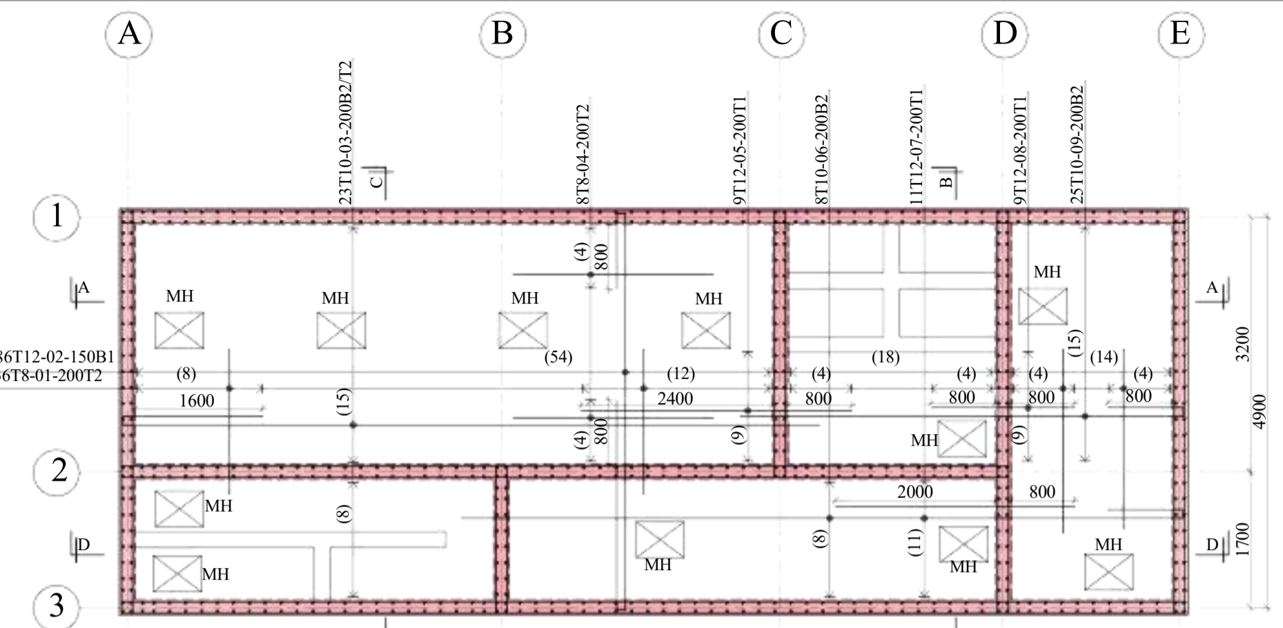
TOP SLAB R.C DETAILS 175MM THICK- (SCALE 1:50)
