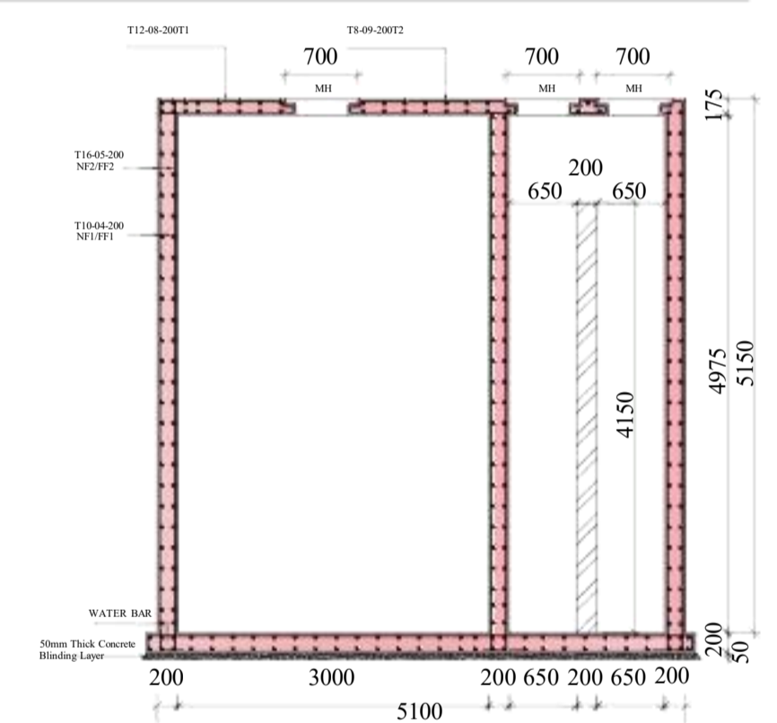
SECTION C-C
