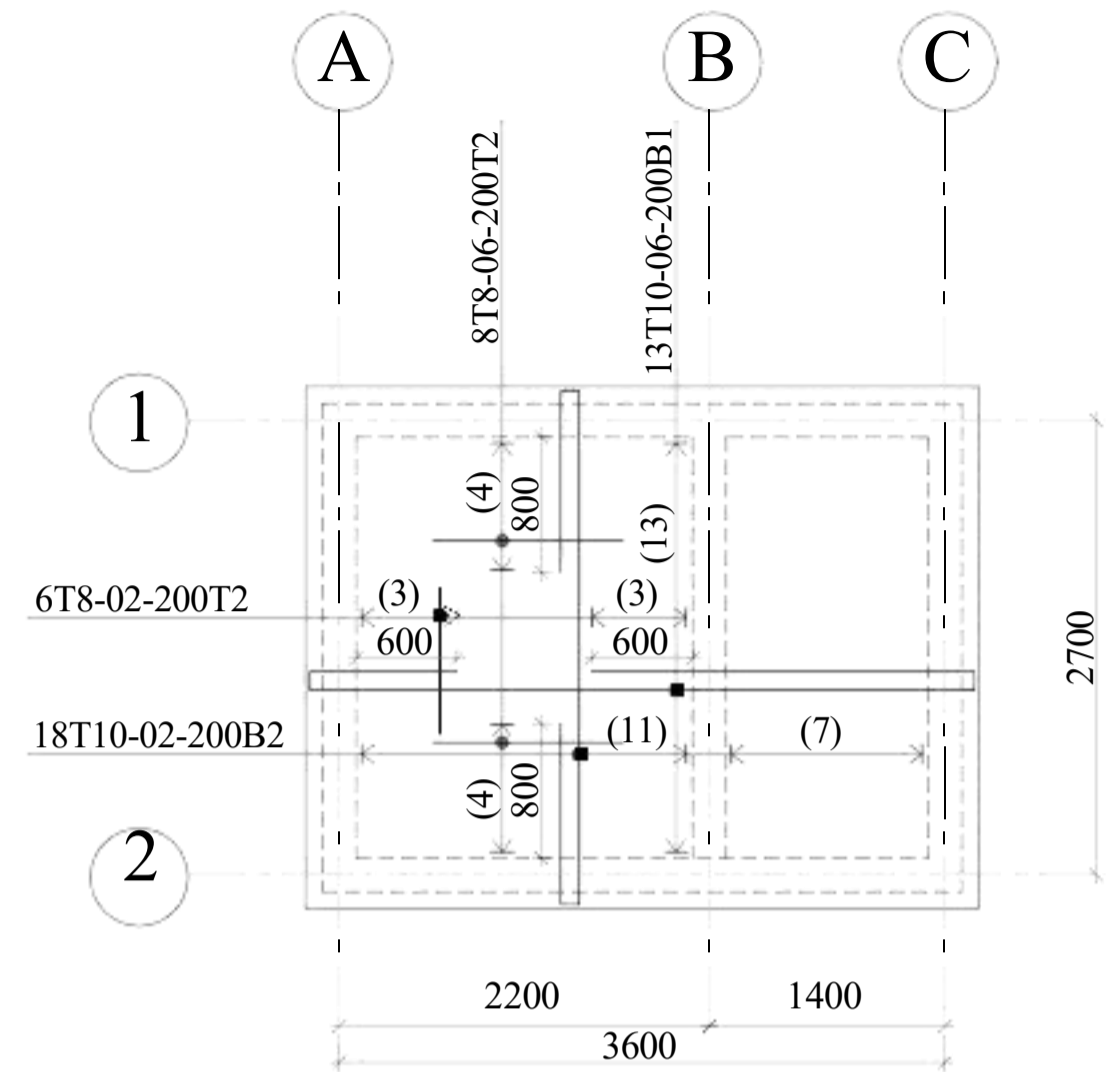
ROOF SLAB R.C DETAILS (1:50)
