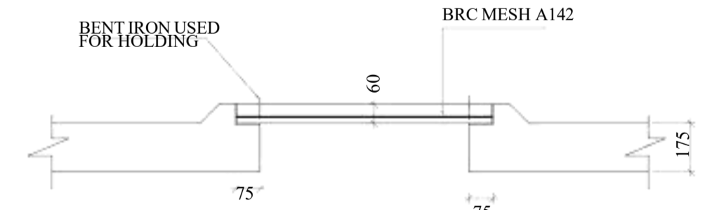
SECTION THROUGH COVER TO 600X600 MANHOLE
