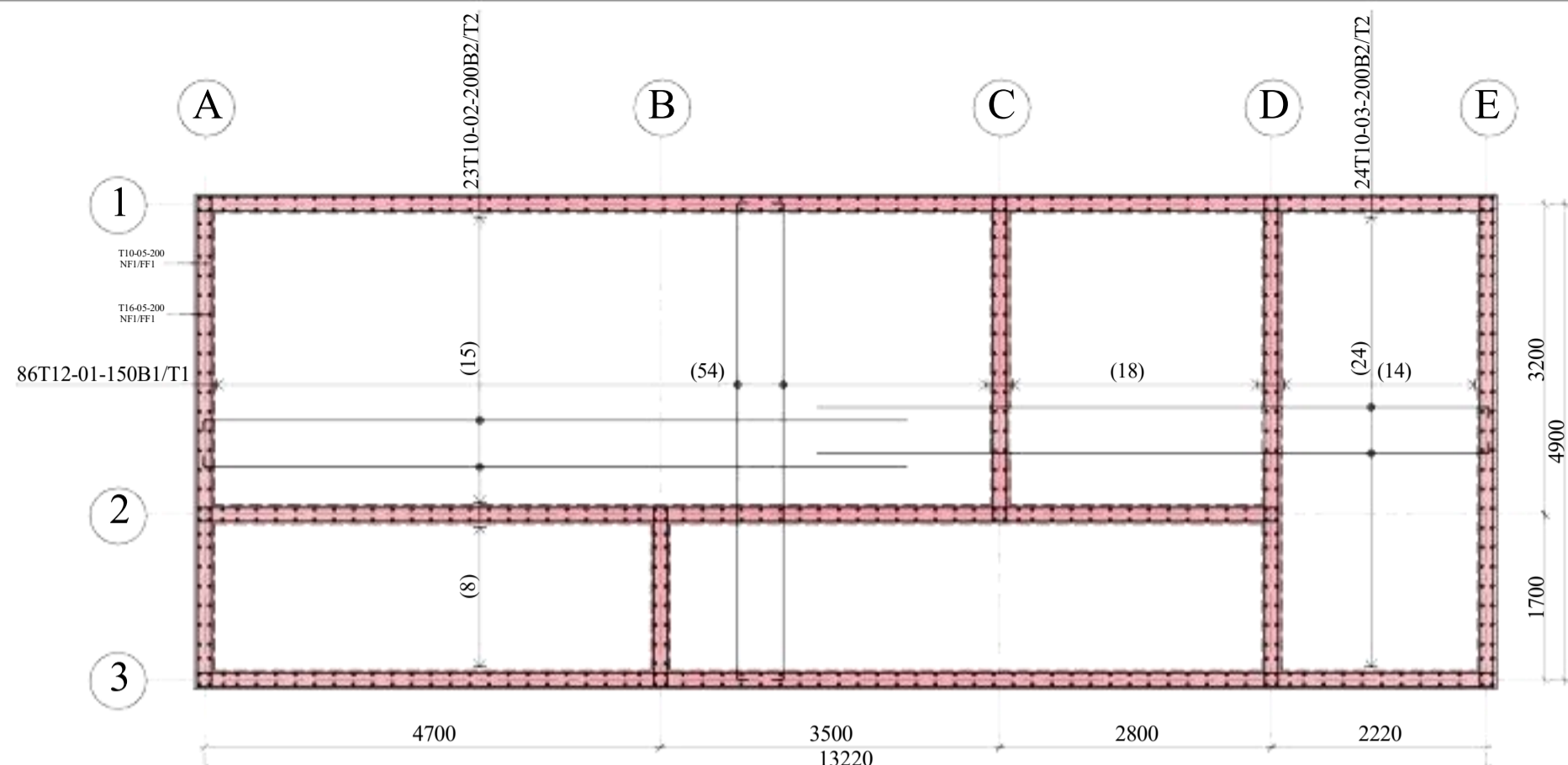
FOUNDATION SLAB R.C DETAILS (SCALE 1:50)
