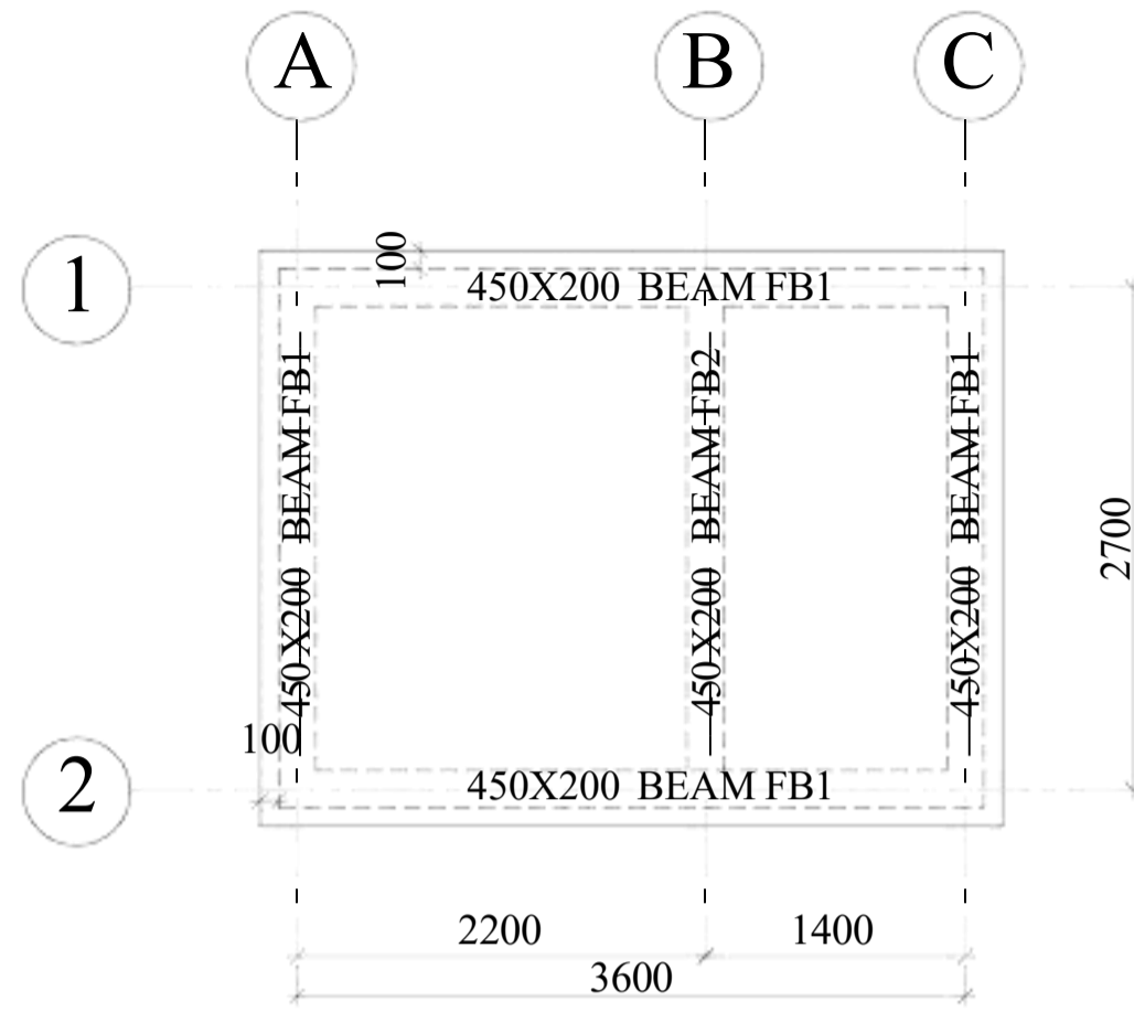
ROOF SLAB BEAMS LAYOUT (1:50)
